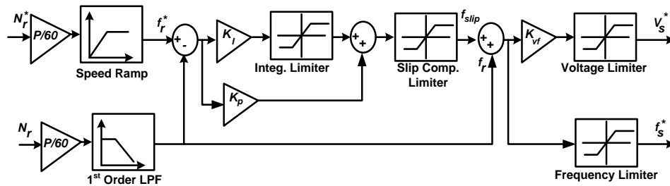
Fig.5 The master controller (sequence of scalar speed control V/f block diagram )
