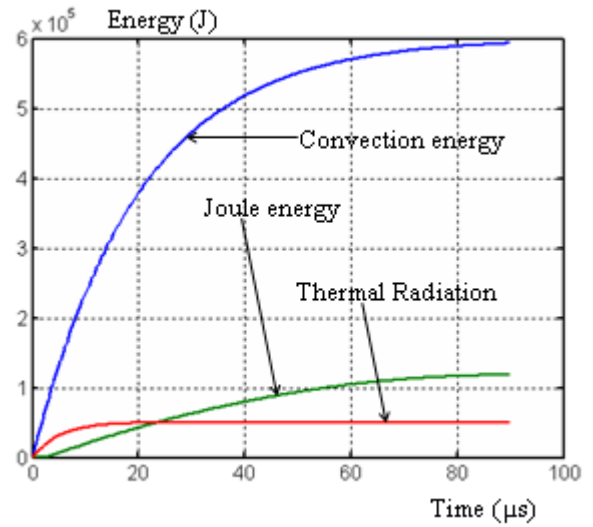
Fig.5: Thermal transfer for \tau = 0.27 \mu s
