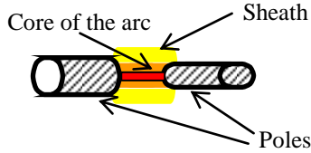
Figure 1. Thermal structure of an arc in SF6
