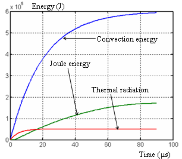
Fig. 6: Thermal transfer for \tau = 0.57 \text{ microseconds}
