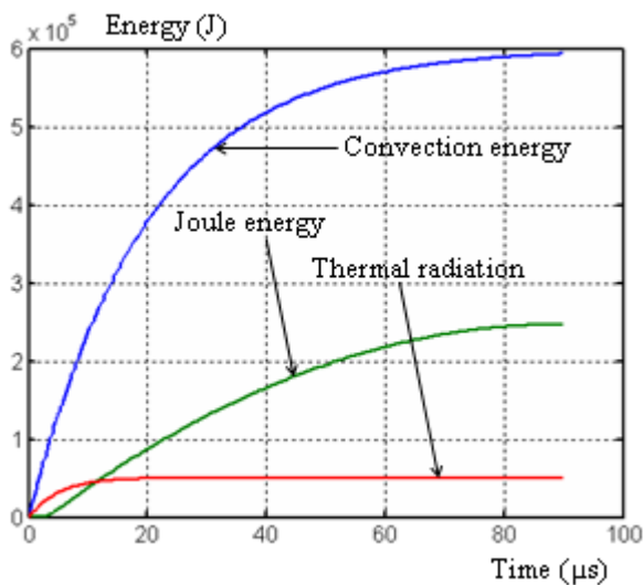
Fig. 7: Thermal transfer for \tau = 1.2\mu s
