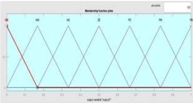
Fig.8.(c) Fuzzy Logic Output
