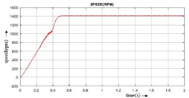
Fig.12. Speed of the motor with PI controller
