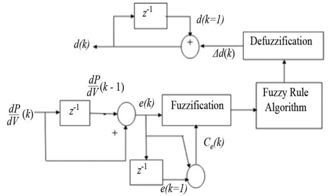
Fig.9. Structure of Fuzzy Logic Controller
