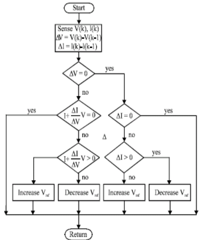
Fig. 7. Flowchart for Incremental conductance algorithm
