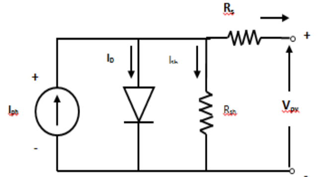
Fig.2. Solar PV cell equivalent circuit
