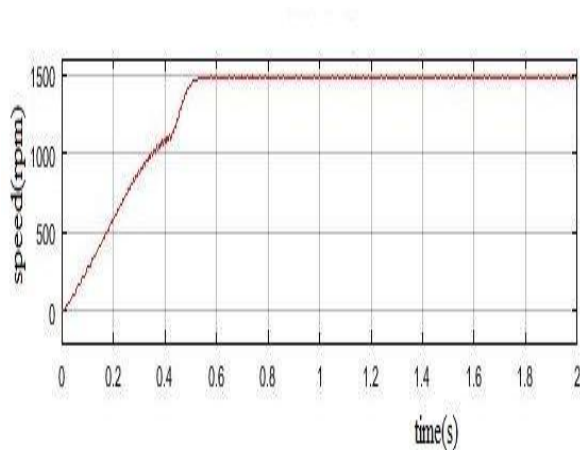
Fig.14. Speed of the motor with neural network controller
