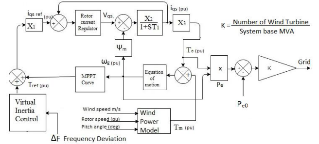
Fig 5. PMSM-WTG model
