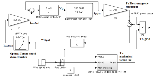
Fig 8. MATLAB/ SIMULINK model for IG- WTG
