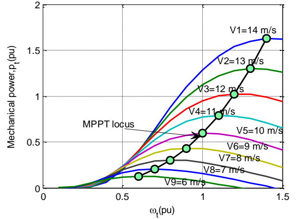
Fig 2. Power –Speed curve
