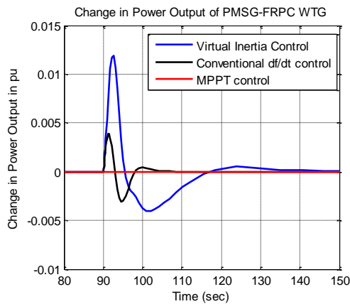
Fig 18. The inertial response of the PMSG-FRPC WTG
