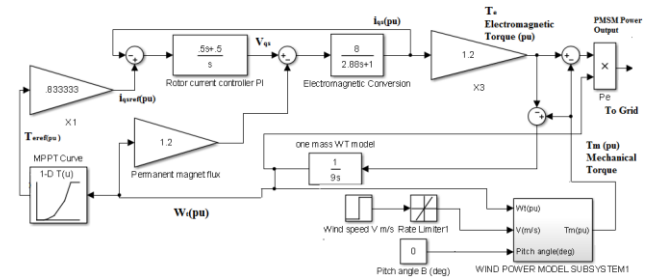
Fig 6. MATLAB/ SIMULINK model for PMSM-WTG
