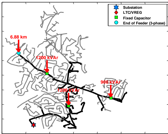
Fig. 2. Topography and major components of distribution test system
