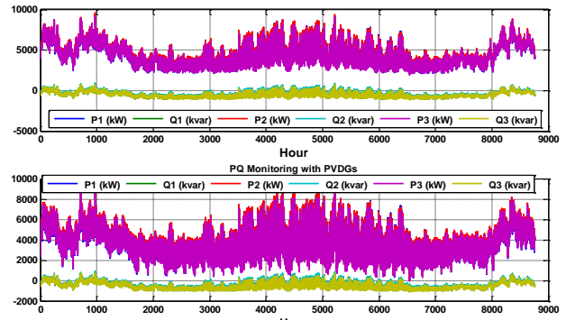
Fig. 7. Yearly substation load with and without PVDG
