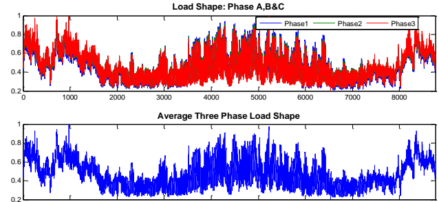
Fig. 3. Yearly profiles of load shapes of Ckt 24 network
