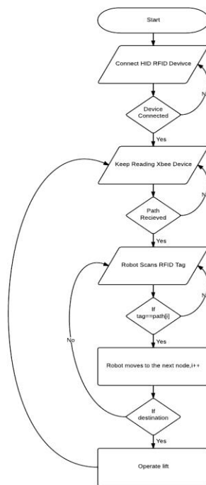
Figure 14 Mbed Code Flowchart
