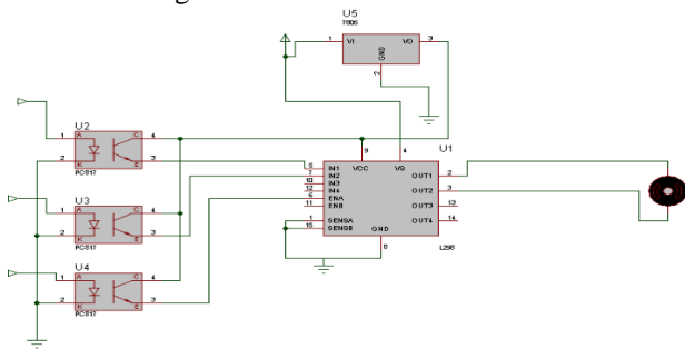
Figure 9 H-Bridge Circuit
