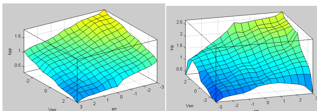
Fig. 62. Output variables surface of K_p and K_i .
