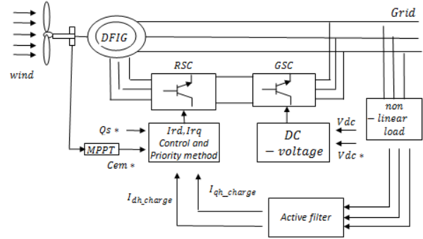
Fig. 1. Block diagram of the wind power system based in DFIG.
