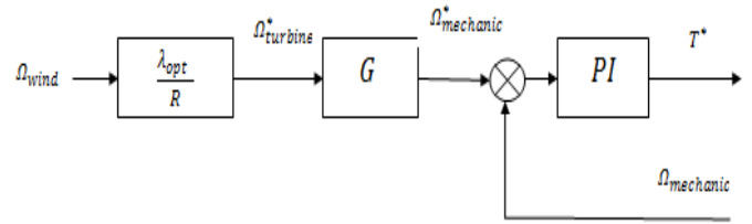
Fig. 2. MPPT control.
