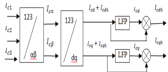
Fig. 6. Block diagram of SRF method.
