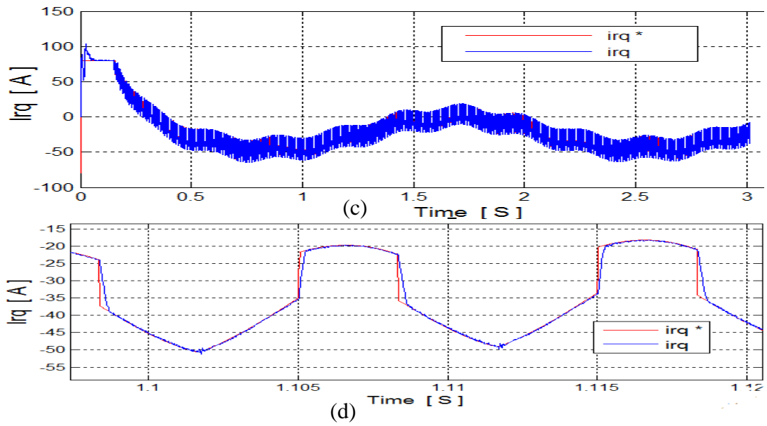
Fig. 7. Rotor currents waveforms: (a) I_{rd} , (b) zoom of I_{rd} , (c) I_{rq} , (d) zoom of I_{rq} .
