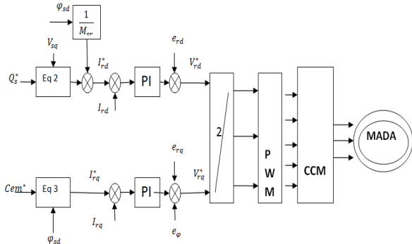
Fig. 3. Block diagram for the RSC control.
