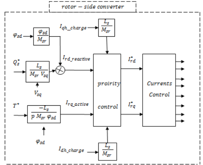
Fig. 5. Modified Rotor-Side Converter Control (MRSC).
