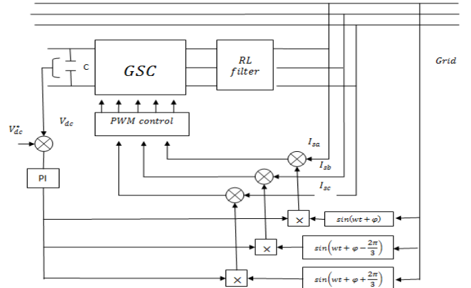
Fig. 4. Block diagram for the GSC control.
