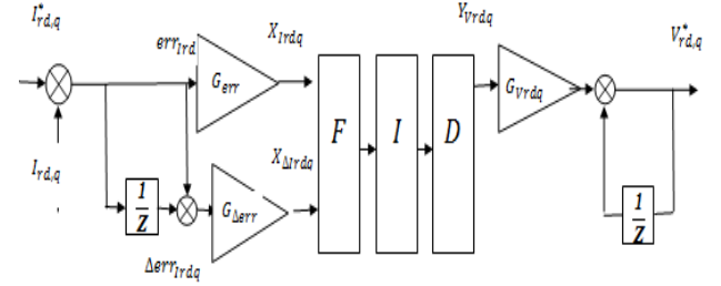
Fig. 10. Bloc diagram of the currents control controller.
