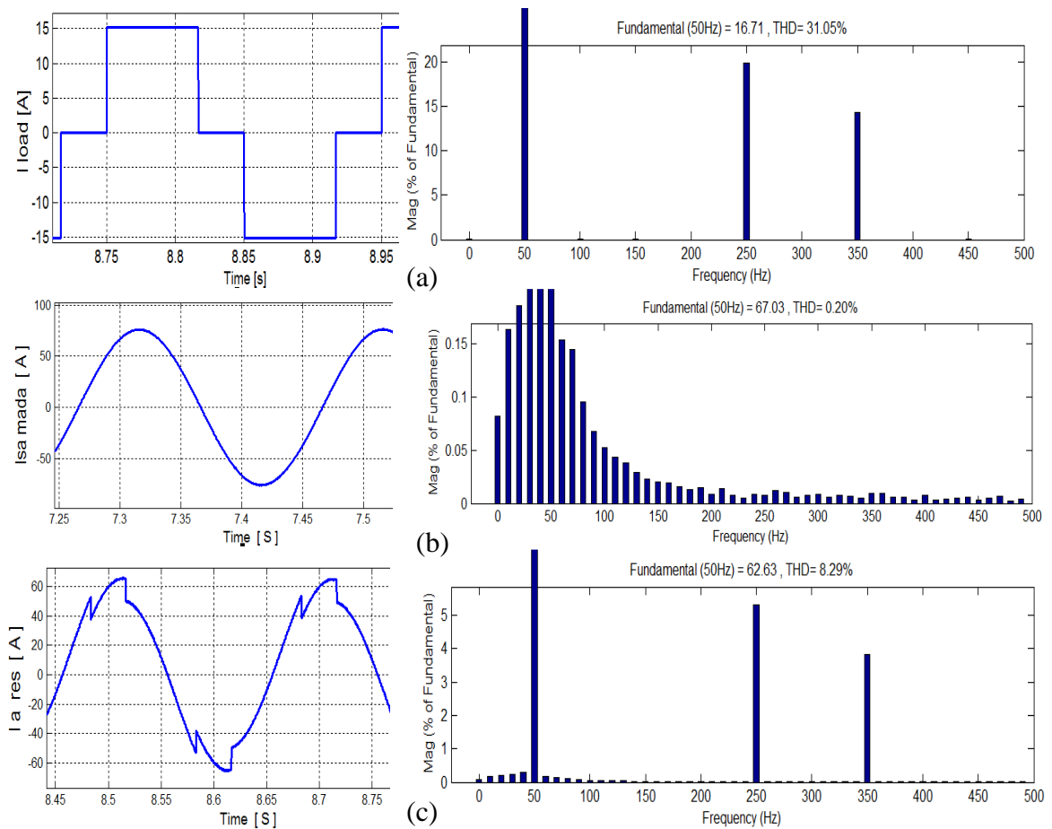
Fig. 8. Current waveforms and their FFT (a) non-linear load, (b) grid, (c) generator
