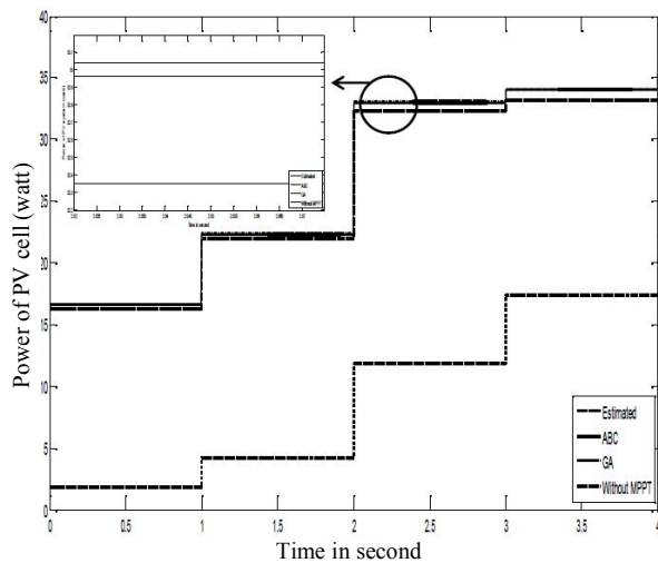
Fig. 15. Power of PV cell for different radiation and temperature.
