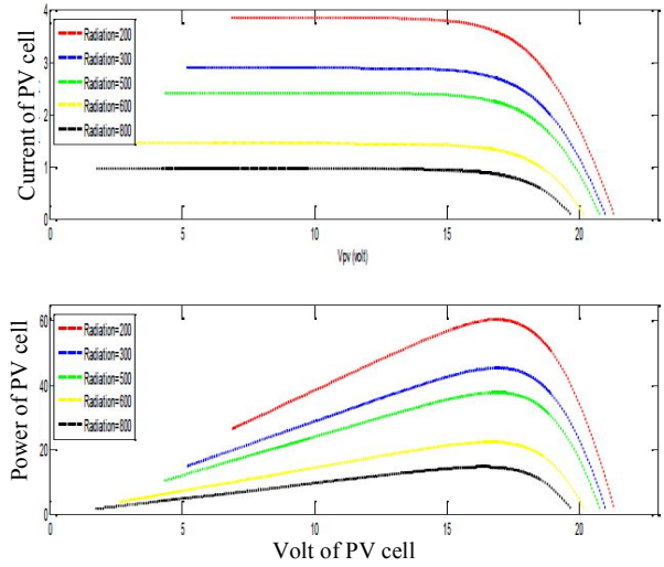
Fig. 6. Relation between volt, current, and power for different radiation.
