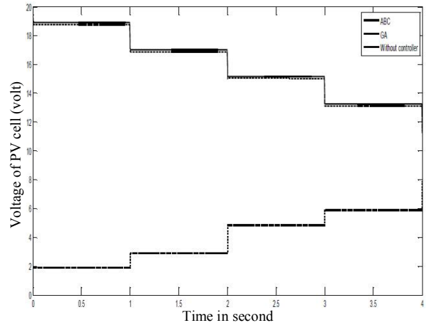
Fig. 16. Change of PV cell voltage for different radiation and temperature.
