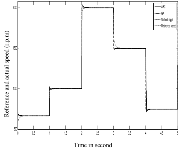
Fig. 20. Change of speed for various controllers.
