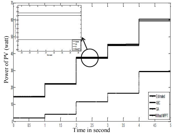
Fig. 7. Power of PV cell for different controllers.
