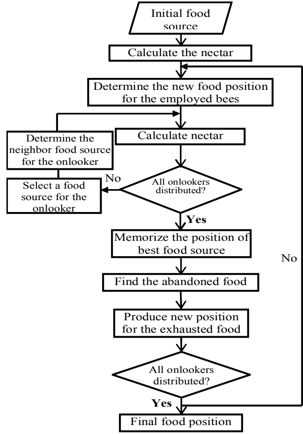
Fig. 3. Flowchart of the ABC algorithm.
