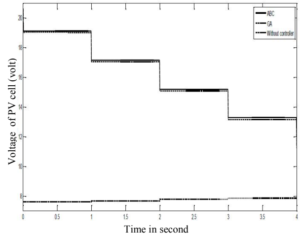
Fig. 12. Voltage of PV cell.
