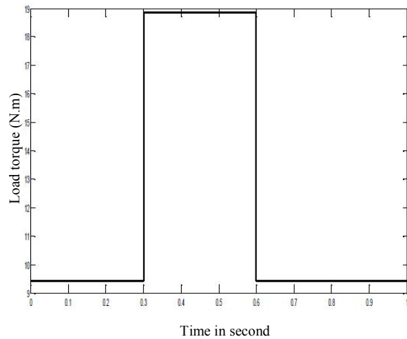
Fig. 17. Change of load torque.
