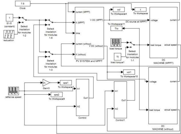
Fig. 2. Overall Matlab system of DC control system supplied by PV system at MPPT.
