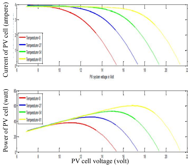
Fig. 10. Change of PV parameters with different temperature.
