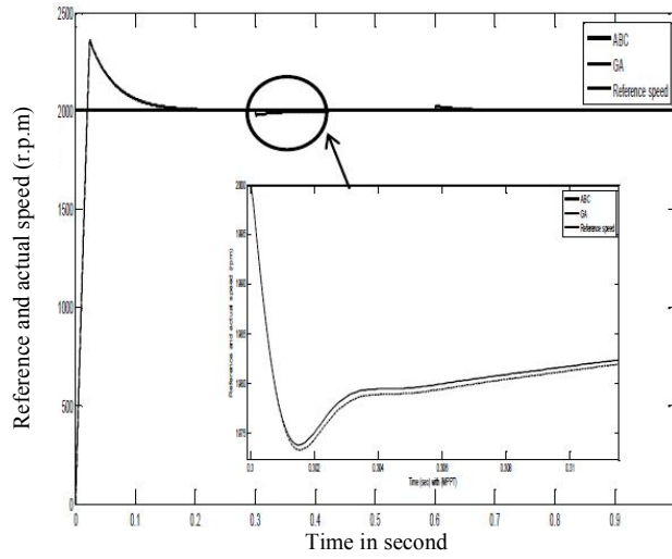
Fig. 18. Change of speed with different controllers.
