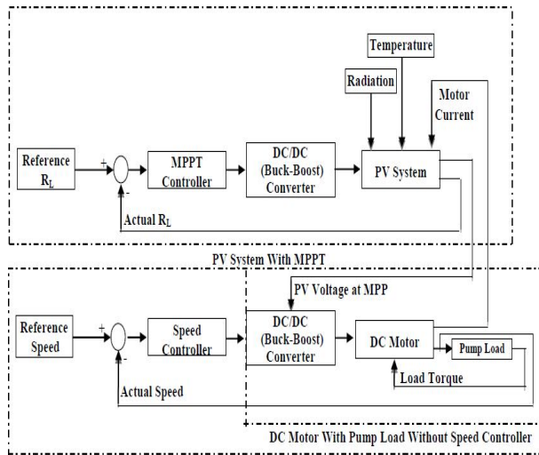
Fig. 1. Overall block diagram of DC control system supplied by PV system at MPPT.
