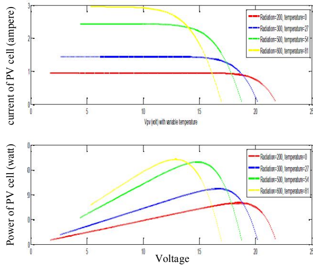
Fig. 14. Change of PV cell parameters with different radiation and temperature.
