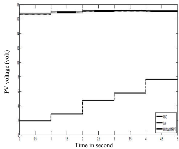
Fig. 8. Voltage of PV cell for different controllers.
