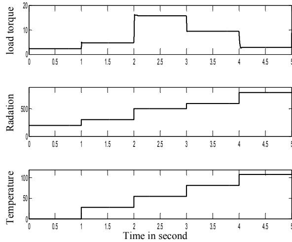
Fig. 19. Change of PV system parameters with load.
