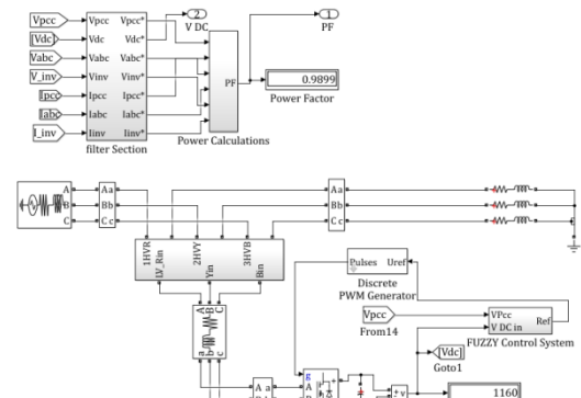
Fig. 16. Implementation of DVR using fuzzy controller with linear load
