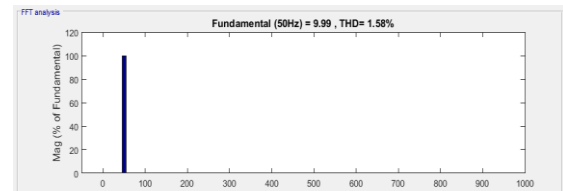
Fig. 24. FFT analysis of load current using fuzzy controller with linear and non-linear load with breaker
