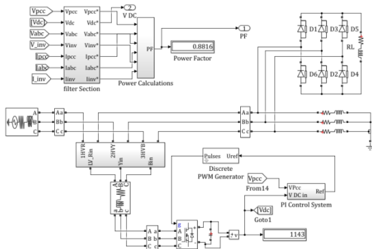
Fig. 13. Implementation of DVR using PI controller with linear and non-linear load without breaker
