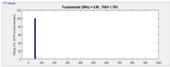
Fig. 15. FFT analysis of load current using PI controller with linear and non-linear load without breaker
