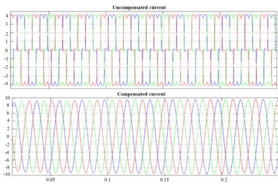
Fig. 20. Load current and compensated current using fuzzy controller with non-linear load
