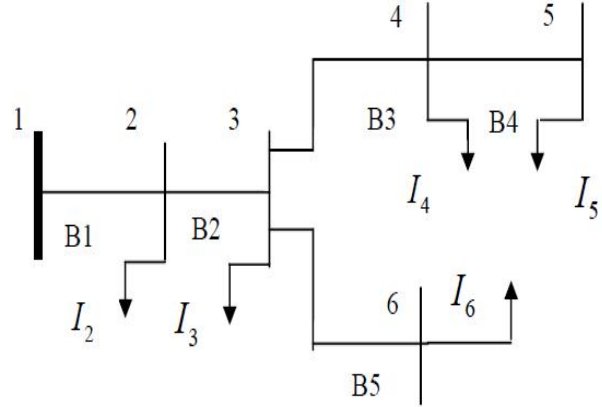
Figure 1 Simple distribution system
