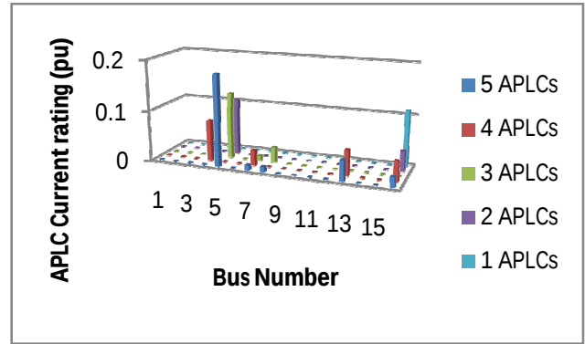
Figure 13 Individual APLC rating in IEEE 18 bus system obtained using DE
