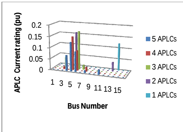
Figure 12 Individual APLC rating in IEEE 18 bus system obtained using HPSOGA
