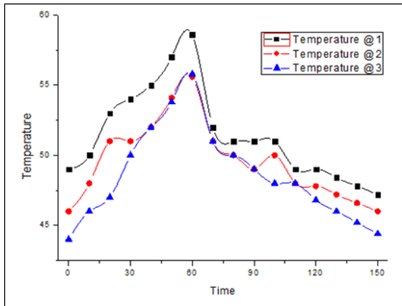
Figure 3. PCM + Graphite at 5 lpm
