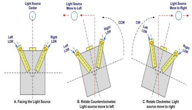
Figure 2: Working Principle of the two LDRs [23]
