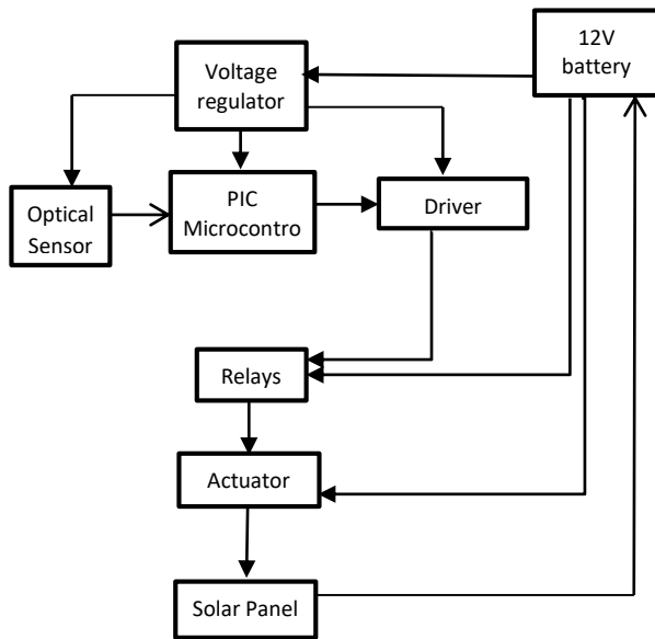
Figure 3: Block diagram of the solar tracking device
