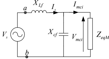
Fig. (5) Steady-state equivalent circuit of matrix converter with its input filter feeding active (induction motor) load.
