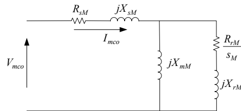
Fig. (4) Per-phase equivalent circuit of an induction motor.
