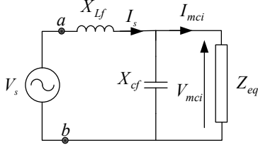
Fig. (1) System under consideration at different loads.
