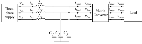
Fig. (1) System under consideration at different loads.
