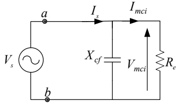
Fig. (3) Reduced steady-state equivalent circuit of the system under consideration.
