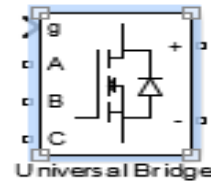
Figure. 4. Three phase MOSFET/DIODE Inverter
