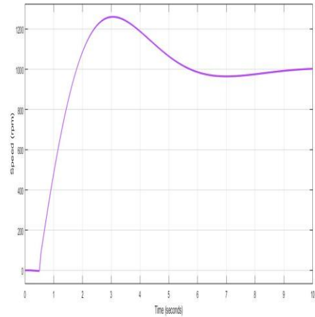
Figure. 10 speed response due to PID controller
