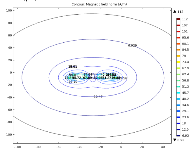
Fig. 6. Magnetic field norm of proposed transceiver at 3MHz ( \frac{A}{m} ).
