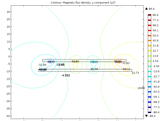
Fig. 5. Magnetic flux density norm of proposed transceiver at 3MHz ( \mu T ).
