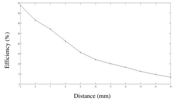
Fig. 18. Power transfer efficiency was measured at distances ranging from 5mm to 15mm while increasing the distance between the coils.
