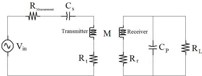
Fig. 3. Equivalent circuit of inductive coupling system.
