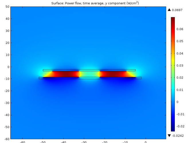
Fig. 8. Power density of proposed transceivers, y component at 3MHz ( \frac{W}{cm^2} ).
