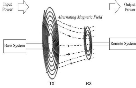
Fig. 1. Near-field transmission technique.
