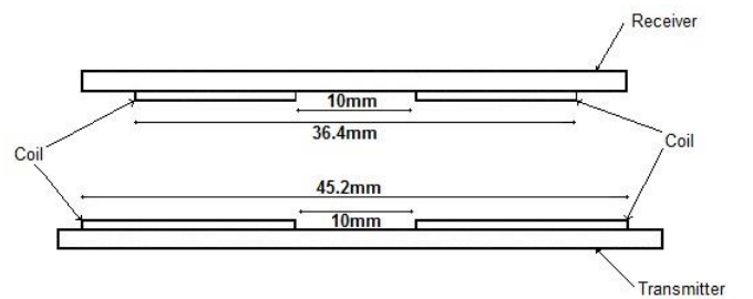
Fig.4. Transceiver.
