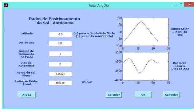
Fig. 3. Construction of MATLAB program on the estimation of anual mean solar radiation and Equivalent Hours of Sun according to day of the year searched.
