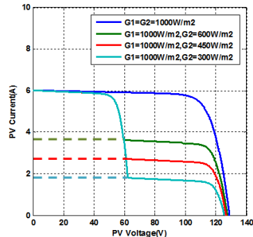
Figure-8 V-I Curves at 25°C
